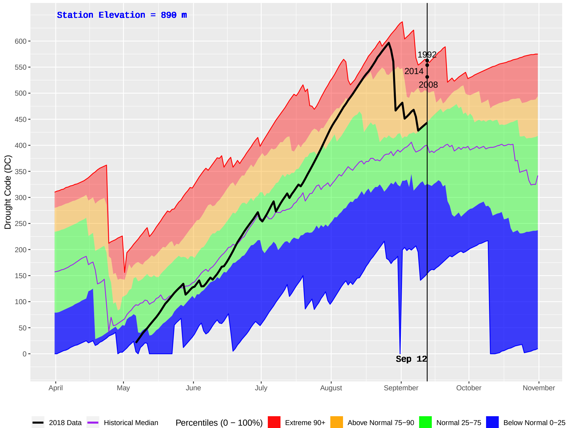
ISKUT (112) : Historical (1979–2016) and Current (2018) Daily Drought Code (DC)
