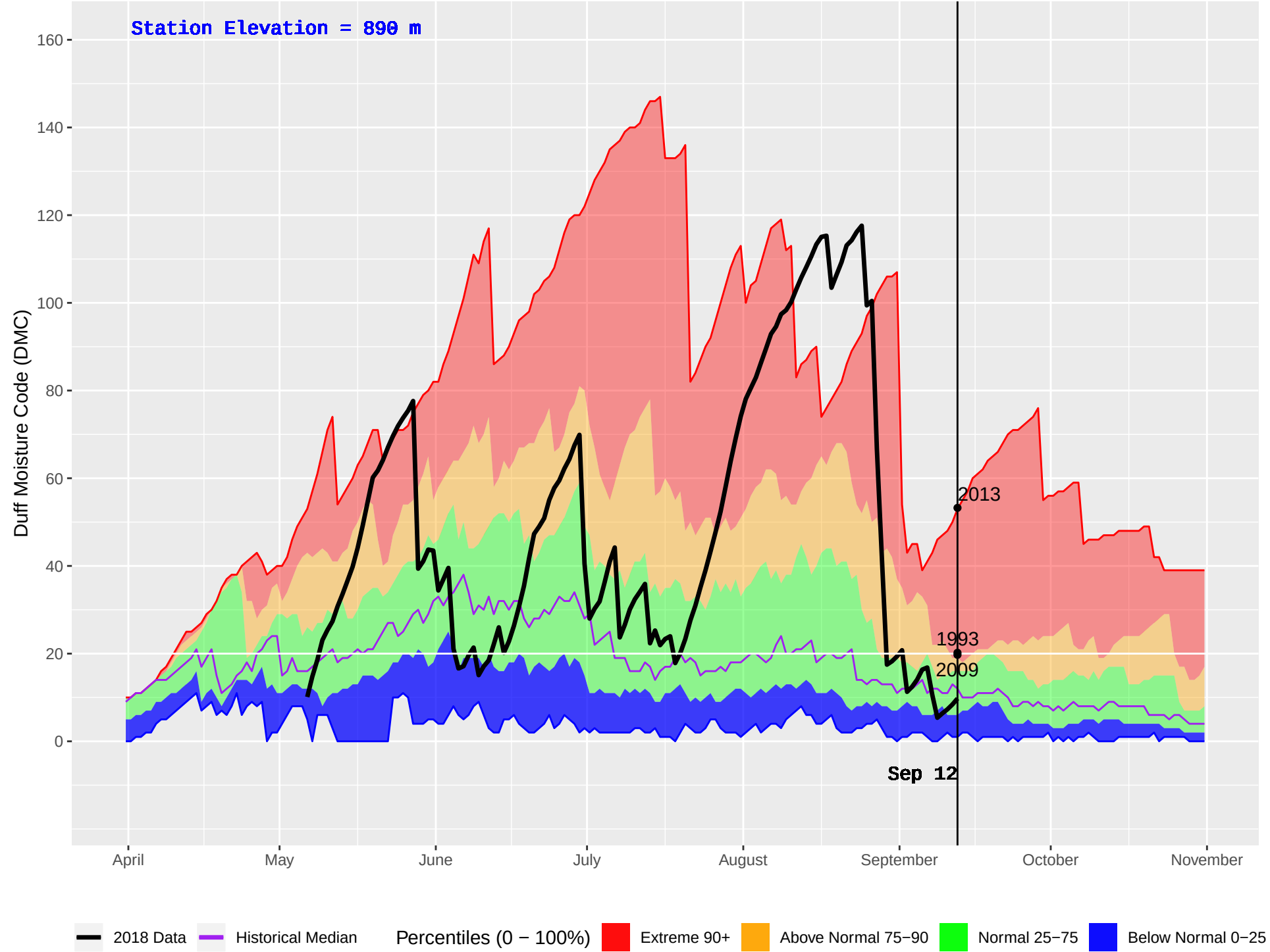
ISKUT (112) : Historical (1979–2016) and Current (2018) Daily Duff Moisture Code (DMC)
