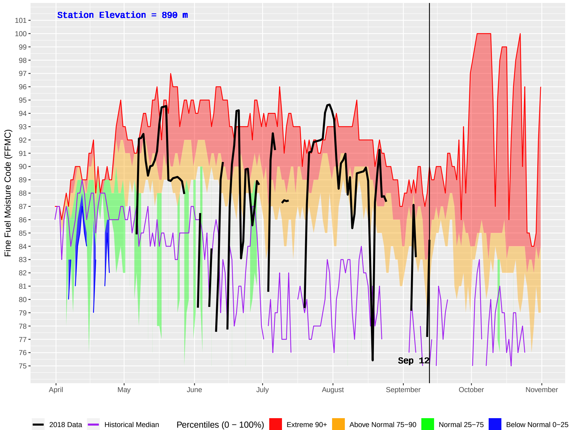
ISKUT (112) : Historical (1979–2016) and Current (2018) Daily Fine Fuel Moisture Code (FFMC)
