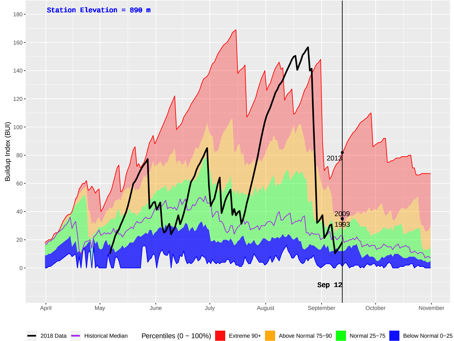
ISKUT (112) : Historical (1979–2016) and Current (2018) Daily Buildup Index (BUI)
