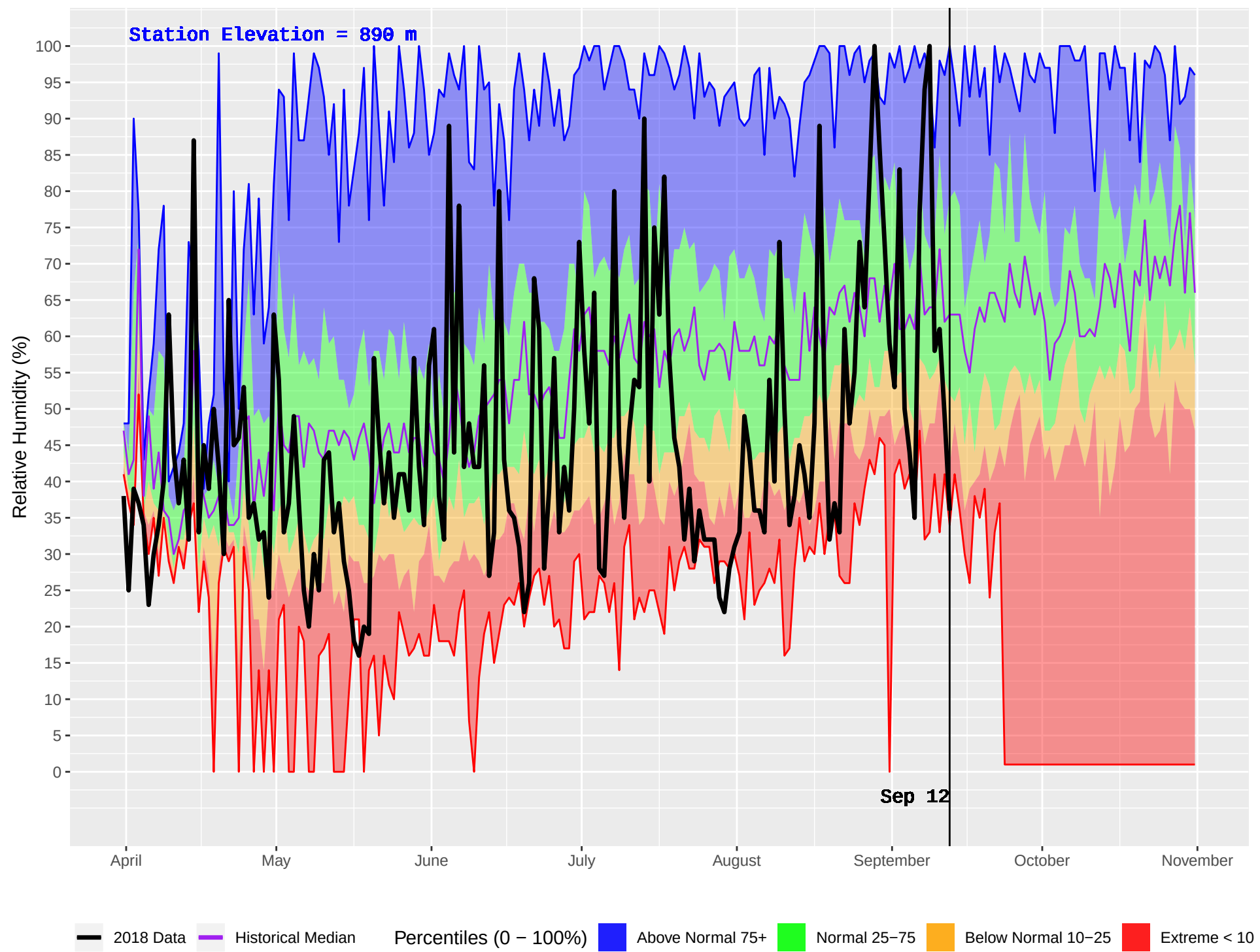
ISKUT (112) : Historical (1979–2016) and Current (2018) Daily Relative Humidity
