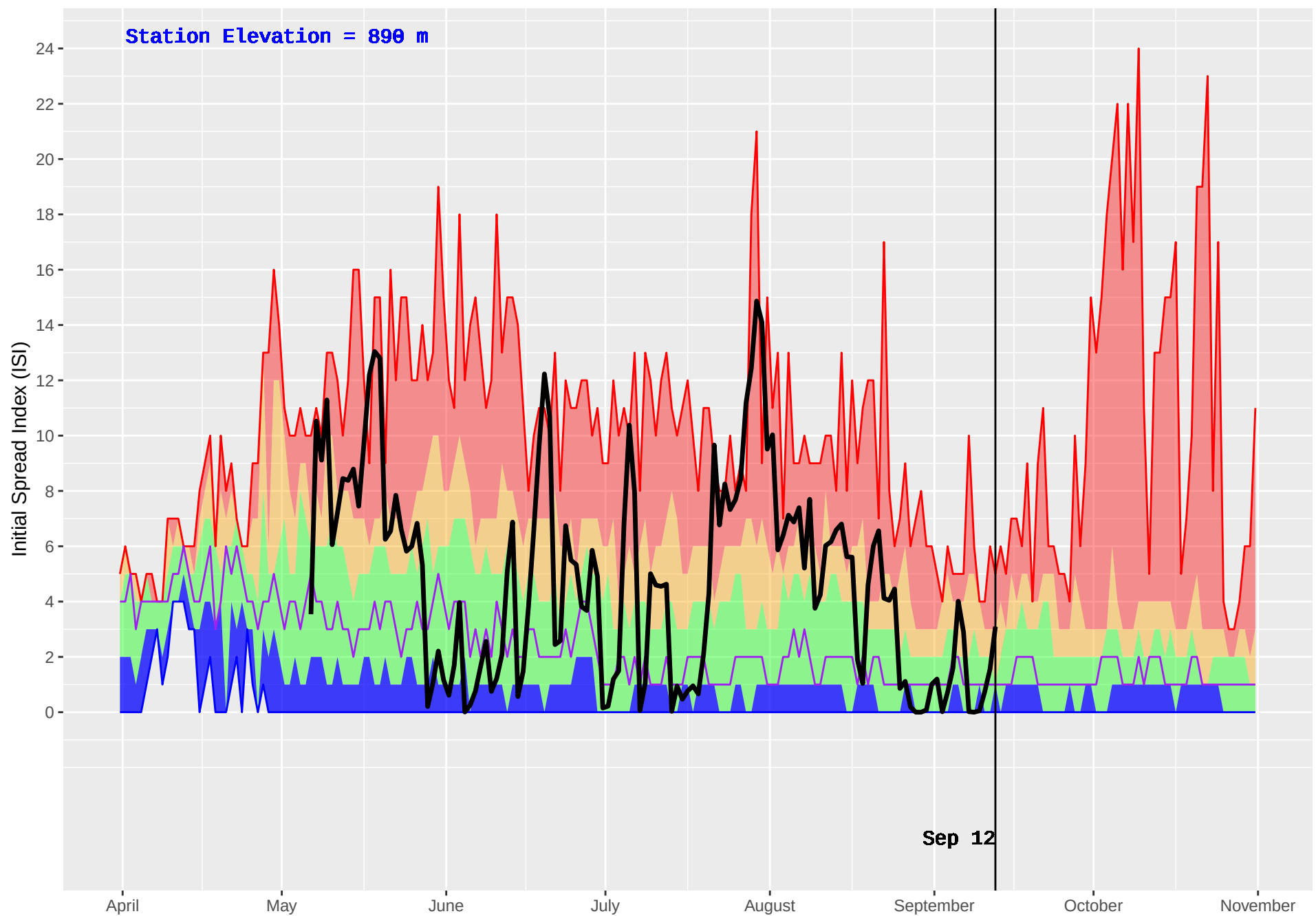
ISKUT (112) : Historical (1979–2016) and Current (2018) Daily Initial Spread Index (ISI)
